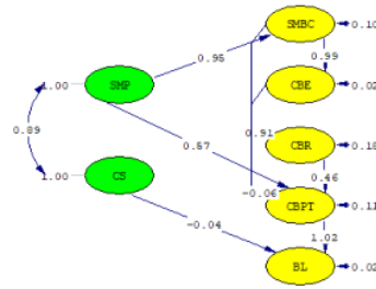
Gambar 1. Path Diagram T-Value
