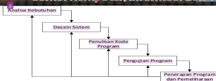
Gambar 1. Metode Waterfall
