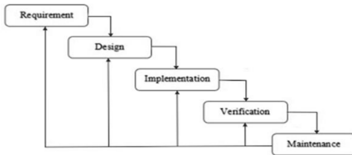
Gambar 1 Metode Waterfall
