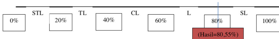
Gambar 8. Presentase Kelayakan
