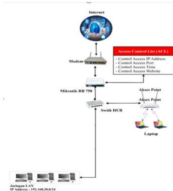
Gambar 1. Blok Diagram Global
