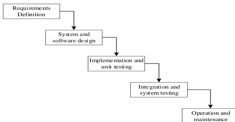
Gambar 1. Metode Waterfall
