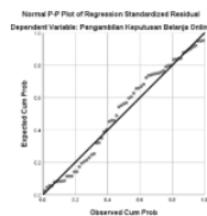
Gambar 1. Normal Probability Plot
